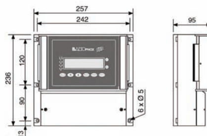
Wall mounting instrument
