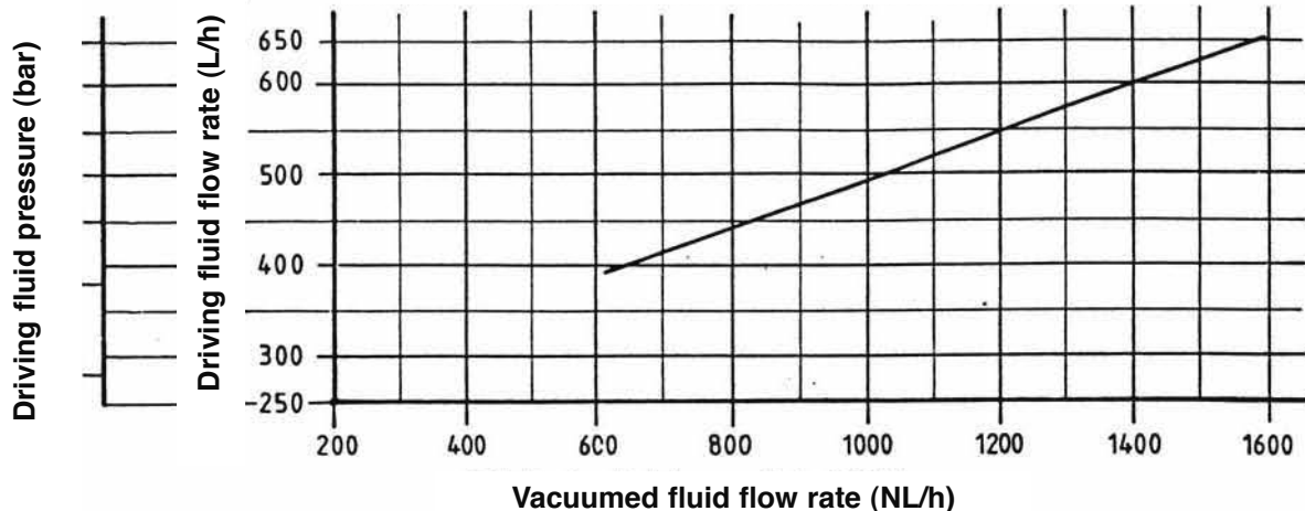
WITH NOZZLE DRILLED BORE Ø 2.5 mm
