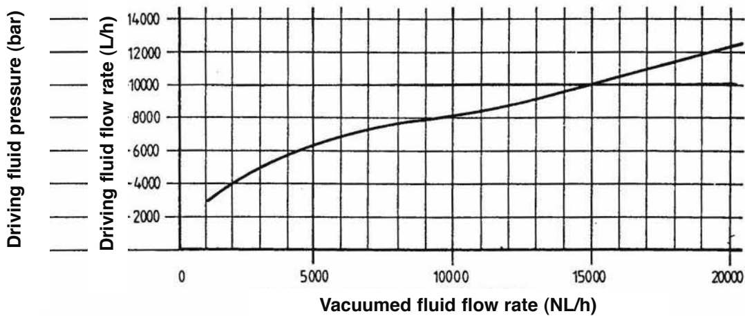
WITH NOZZLE DRILLED BORE Ø 14 mm
