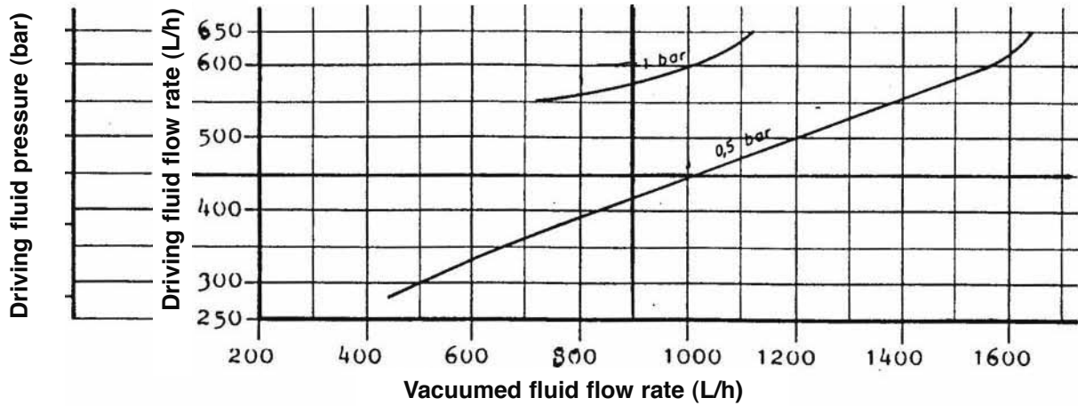
WITH NOZZLE DRILLED BORE Ø 2.5 mm
