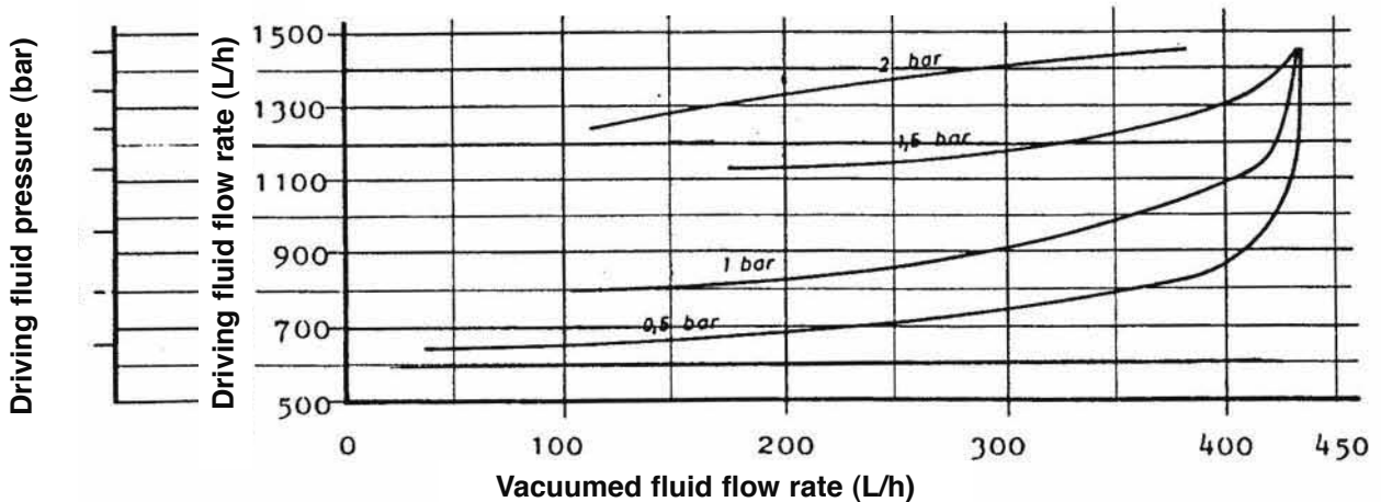
WITH NOZZLE DRILLED BORE Ø 4 mm
