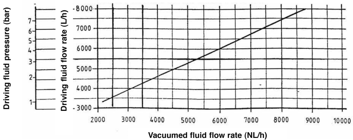
WITH NOZZLE DRILLED BORE Ø 9 mm
