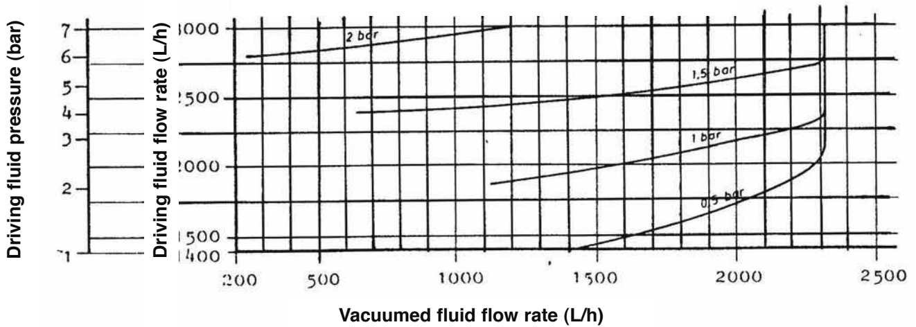
WITH NOZZLE DRILLED BORE Ø 5.5 mm
