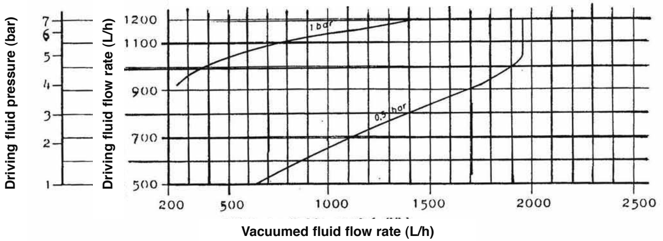
WITH NOZZLE DRILLED BORE Ø 3.5 mm
