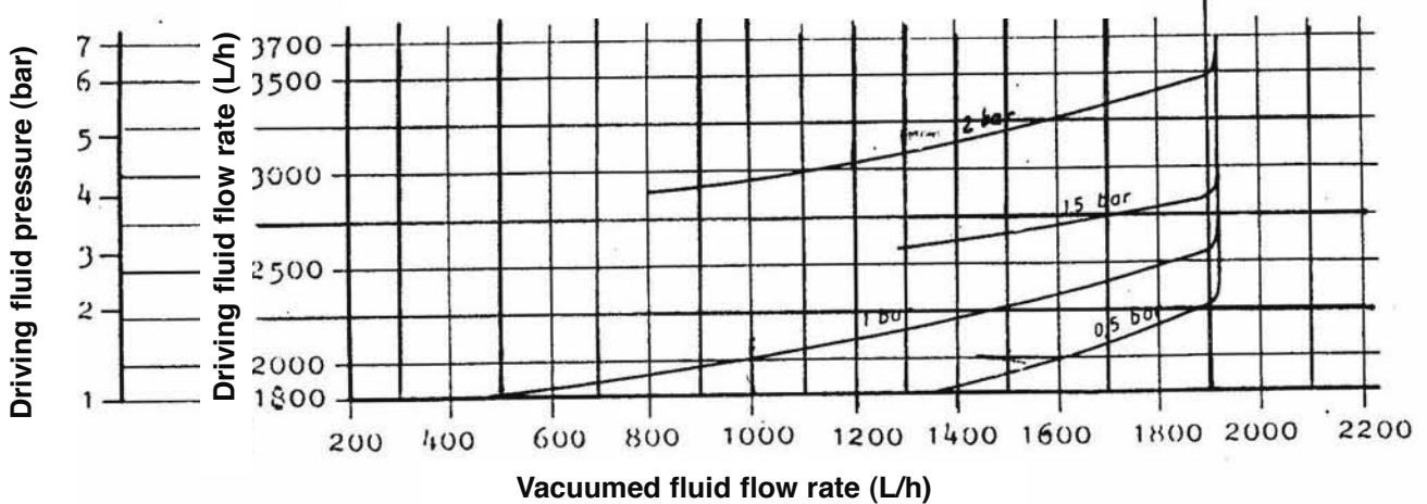
WITH NOZZLE DRILLED BORE Ø 6 mm
