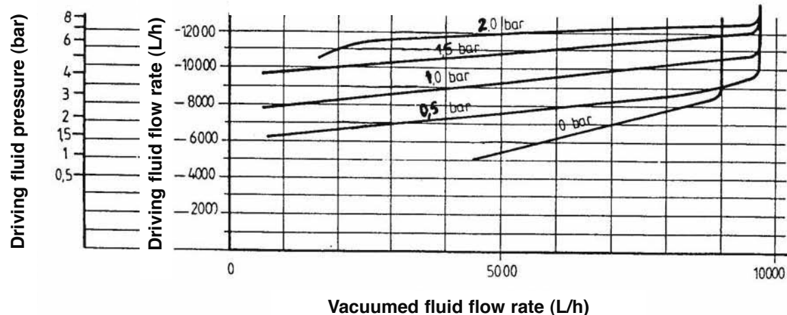
WITH NOZZLE DRILLED BORE Ø 11.5 mm
