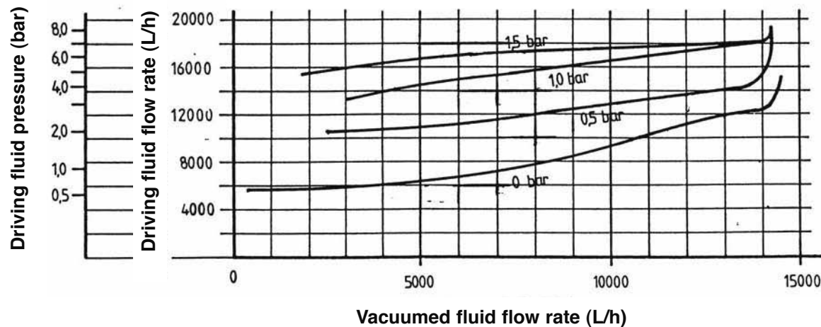
WITH NOZZLE DRILLED BORE Ø 14 mm
