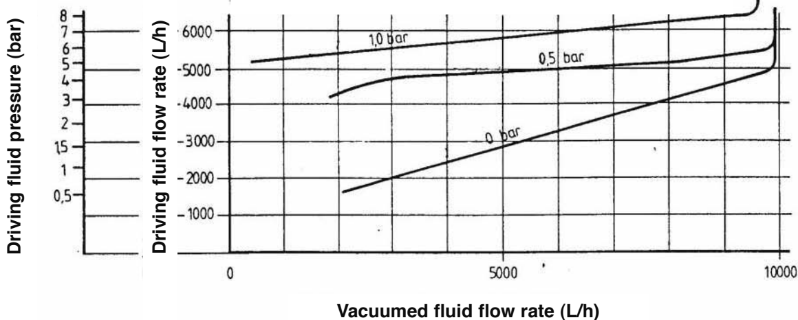
WITH NOZZLE DRILLED BORE Ø 9 mm
