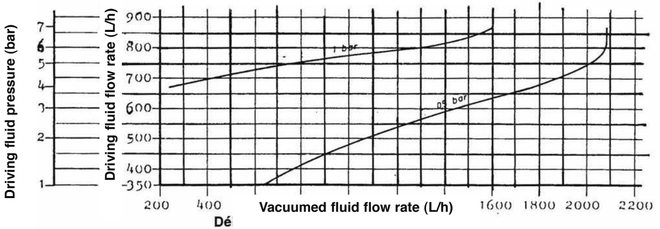
WITH NOZZLE DRILLED BORE Ø 3 mm
