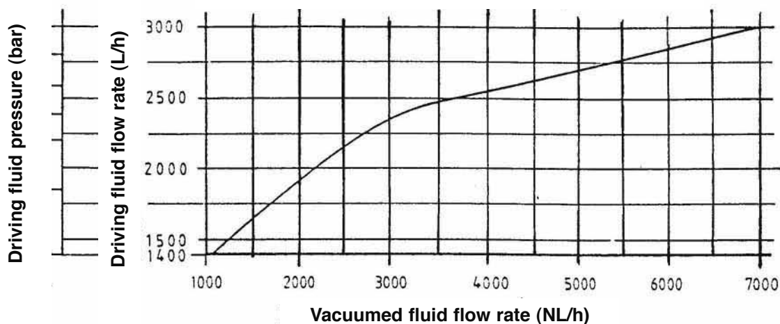
WITH NOZZLE DRILLED BORE Ø 5.5 mm
