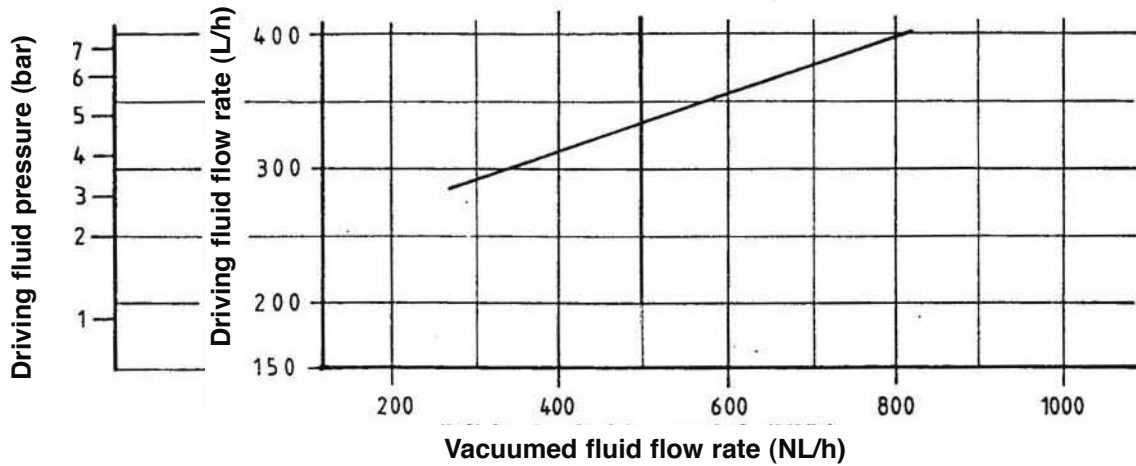
WITH NOZZLE DRILLED BORE Ø 2 mm
