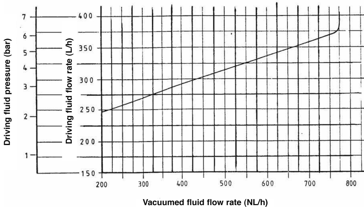
WITH NOZZLE DRILLED BORE Ø 2 mm
