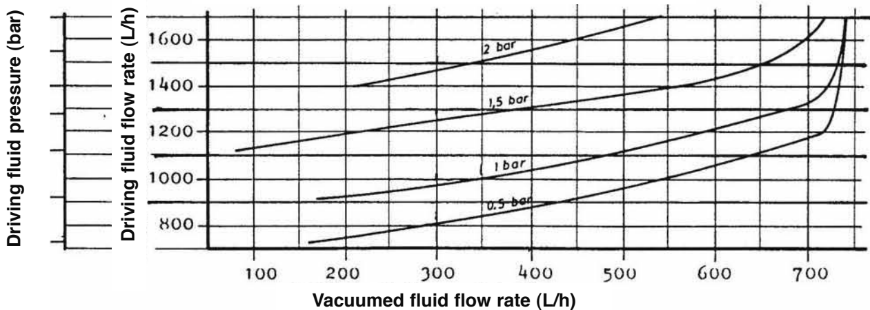
WITH NOZZLE DRILLED BORE Ø 4.5 mm
