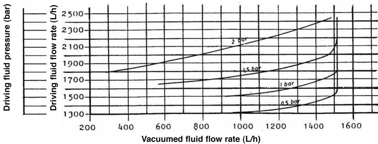
WITH NOZZLE DRILLED BORE Ø 5 mm
