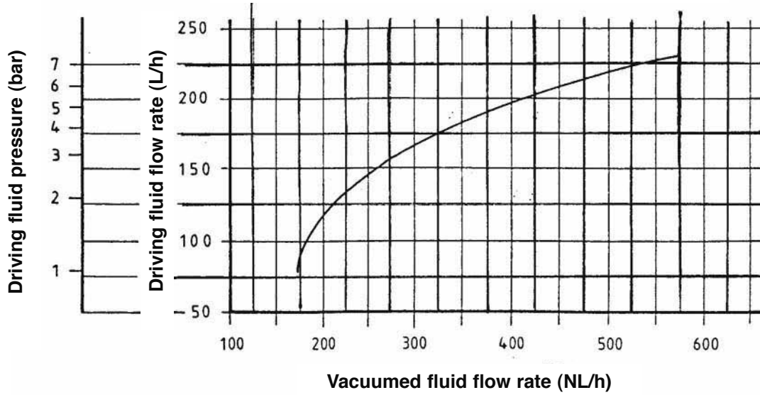
WITH NOZZLE DRILLED BORE Ø 1.5 mm
