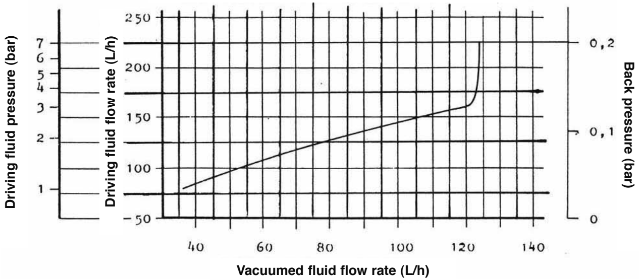
WITH NOZZLE DRILLED BORE Ø 1.5 mm
