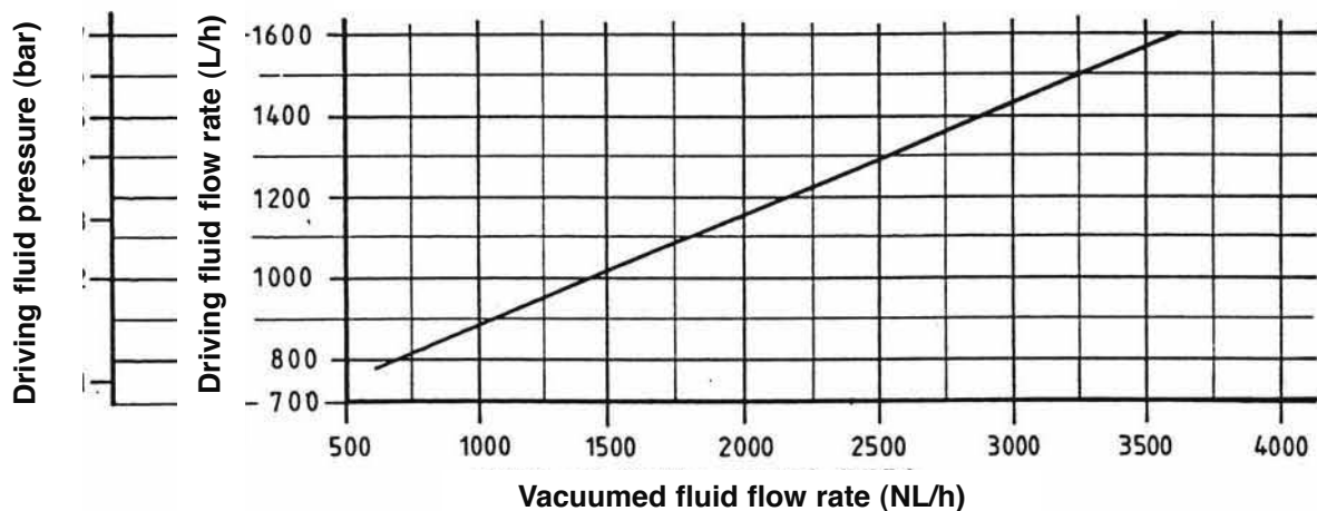
WITH NOZZLE DRILLED BORE Ø 4 mm
