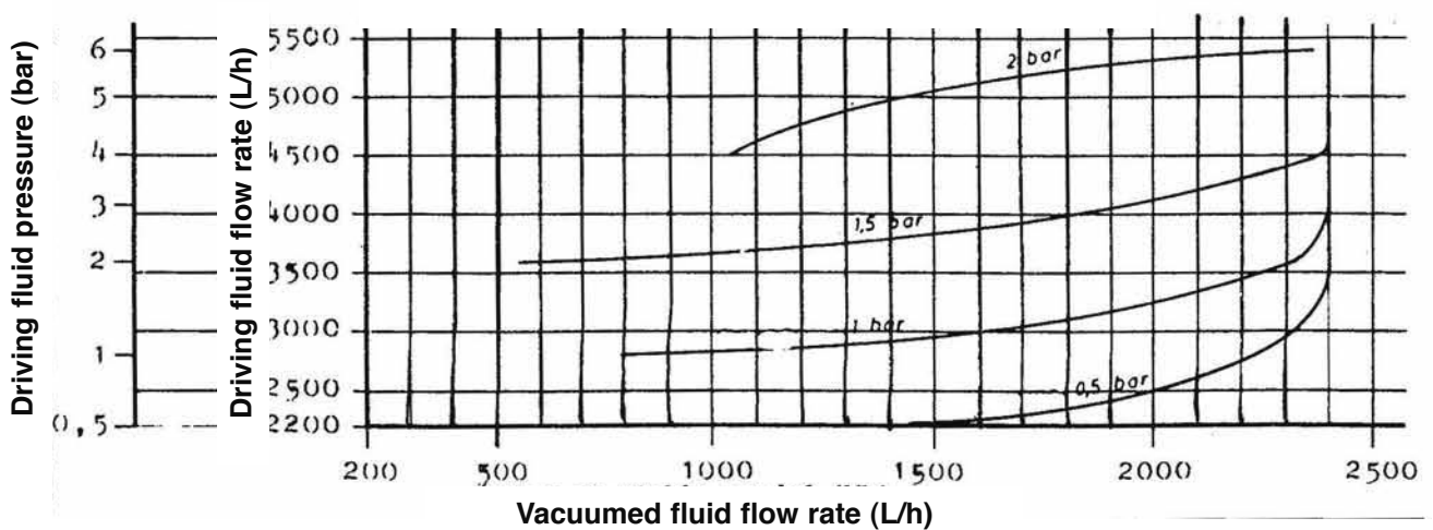
WITH NOZZLE DRILLED BORE Ø 7.5 mm
