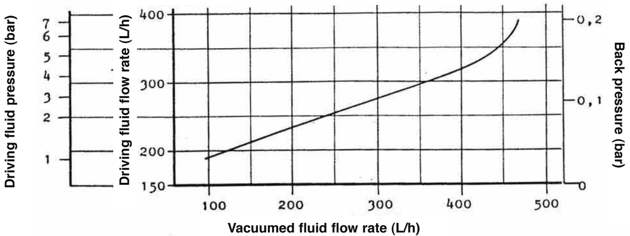
WITH NOZZLE DRILLED BORE Ø 2 mm
