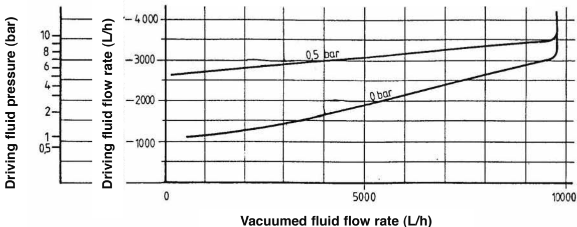
WITH NOZZLE DRILLED BORE Ø 6.5 mm
