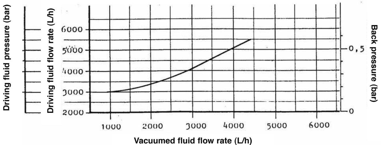
WITH NOZZLE DRILLED BORE Ø 9 mm
