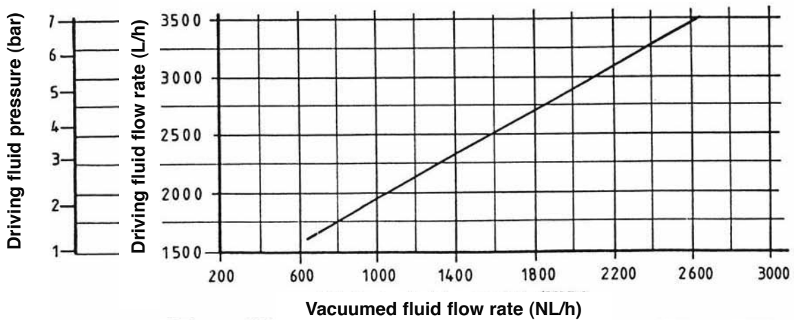
WITH NOZZLE DRILLED BORE Ø 6 mm
