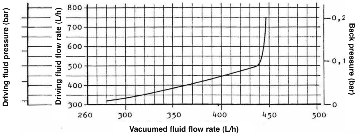
WITH NOZZLE DRILLED BORE Ø 3 mm
