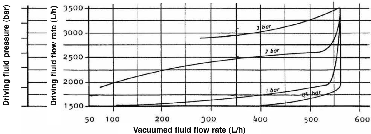
WITH NOZZLE DRILLED BORE Ø 6 mm
