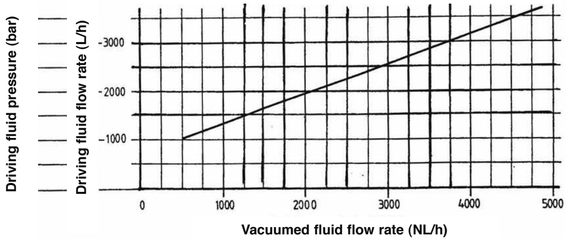
WITH NOZZLE DRILLED BORE Ø 6.5 mm
