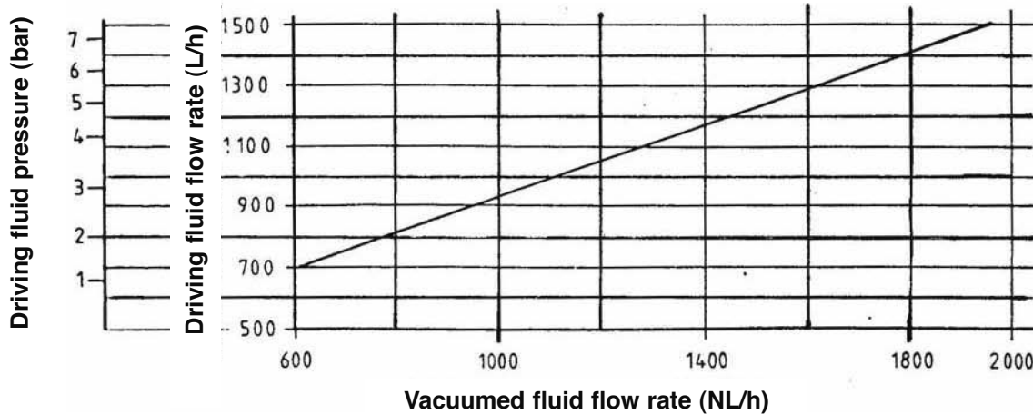
WITH NOZZLE DRILLED BORE Ø 4 mm
