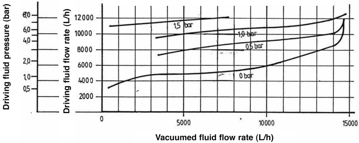
WITH NOZZLE DRILLED BORE Ø 11 mm
