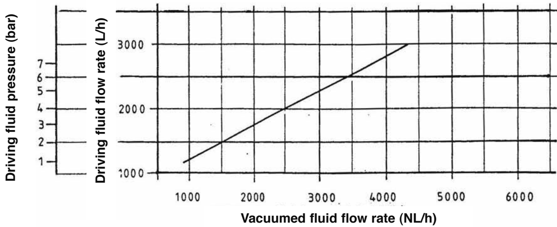
WITH NOZZLE DRILLED BORE Ø 5 mm
