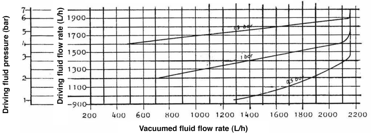
WITH NOZZLE DRILLED BORE Ø 4.5 mm
