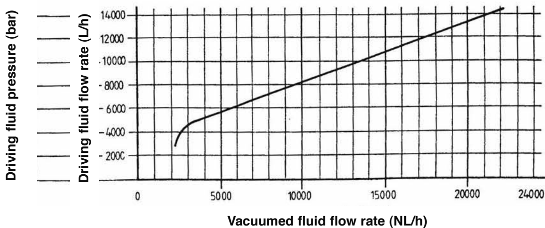
WITH NOZZLE DRILLED BORE Ø 11.5 mm
