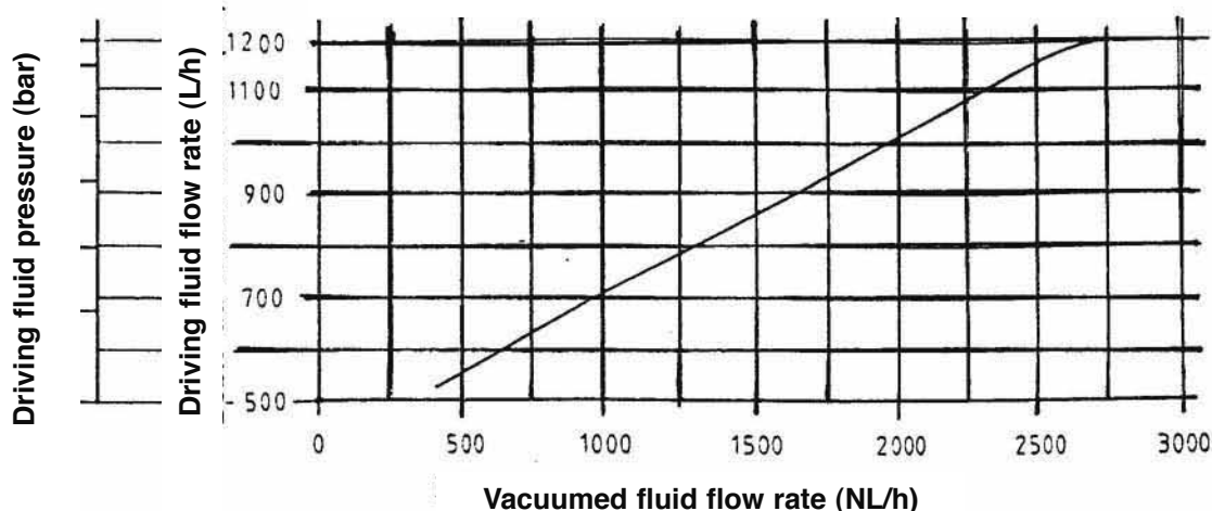
WITH NOZZLE DRILLED BORE Ø 3.5 mm
