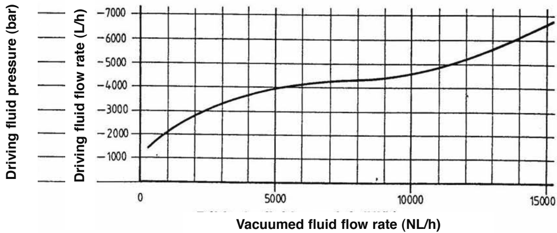
WITH NOZZLE DRILLED BORE Ø 9 mm
