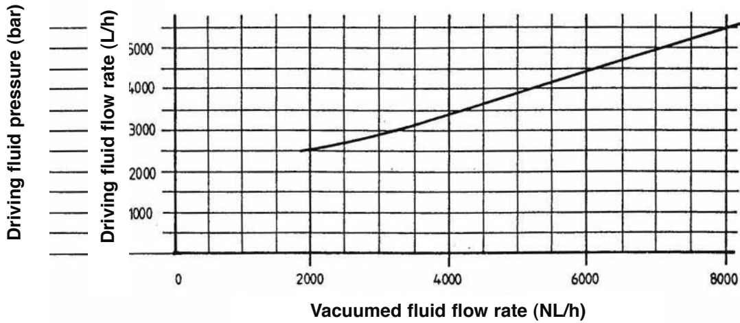
WITH NOZZLE DRILLED BORE Ø 8 mm
