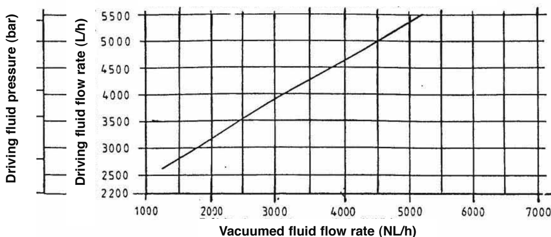
WITH NOZZLE DRILLED BORE Ø 7.5 mm
