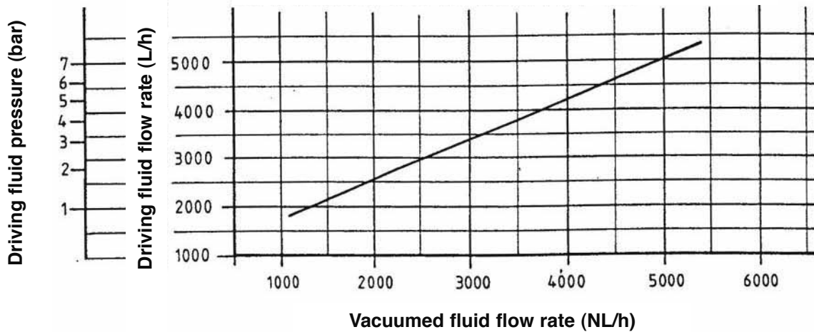
WITH NOZZLE DRILLED BORE Ø 7 mm
