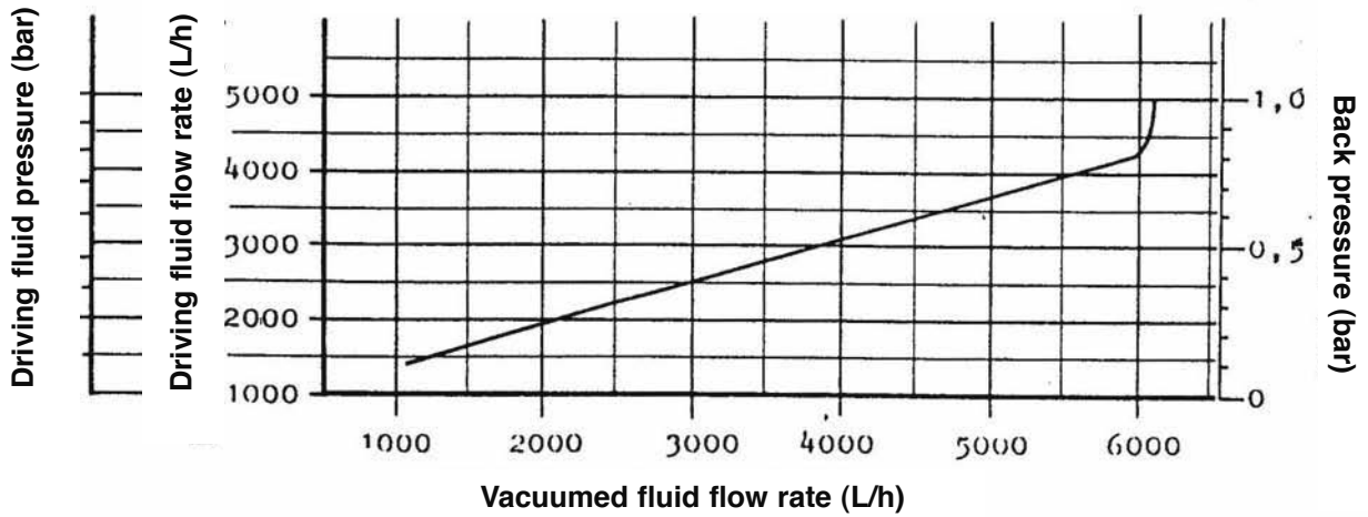
WITH NOZZLE DRILLED BORE Ø 7 mm
