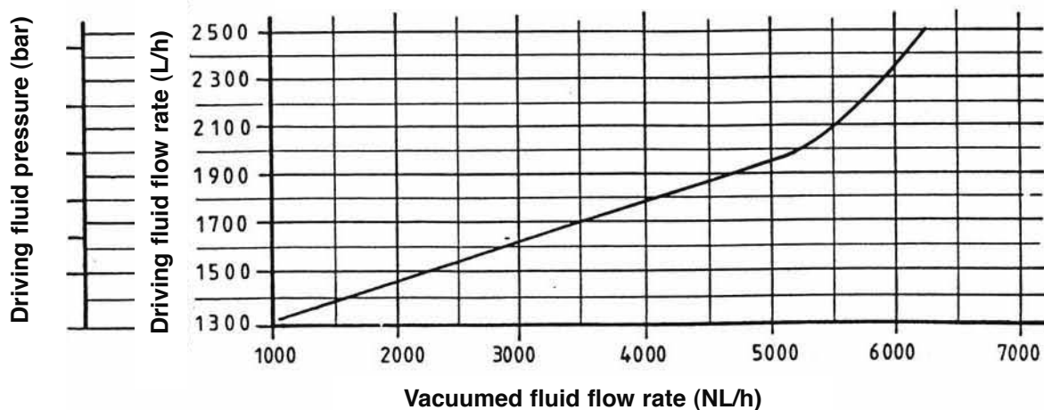
WITH NOZZLE DRILLED BORE Ø 5 mm
