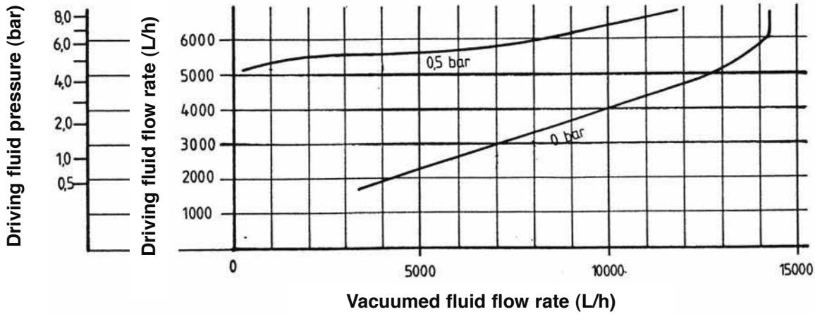
WITH NOZZLE DRILLED BORE Ø 8 mm
